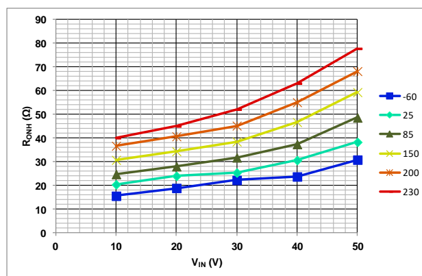
Figure 16. High-state on-resistance of output drivers vs input voltage ( V_{IN} ) for different case temperatures. Device sourcing 10mA, V_{DD}=5V (/LPMMode=1).
