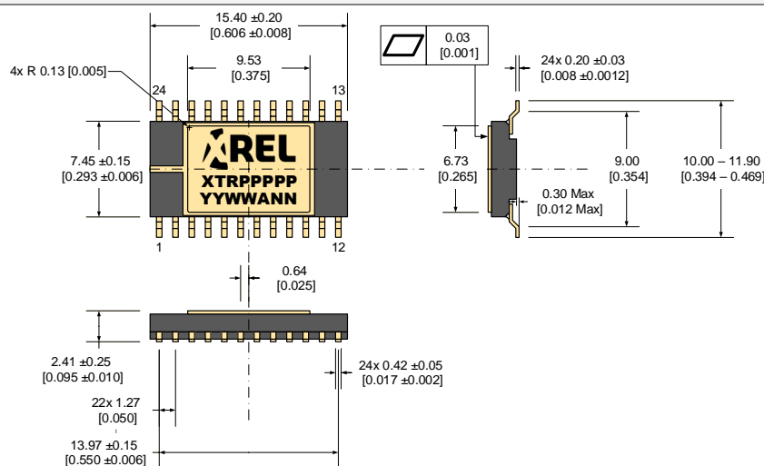
Ceramic Small Outline IC SOIC24
