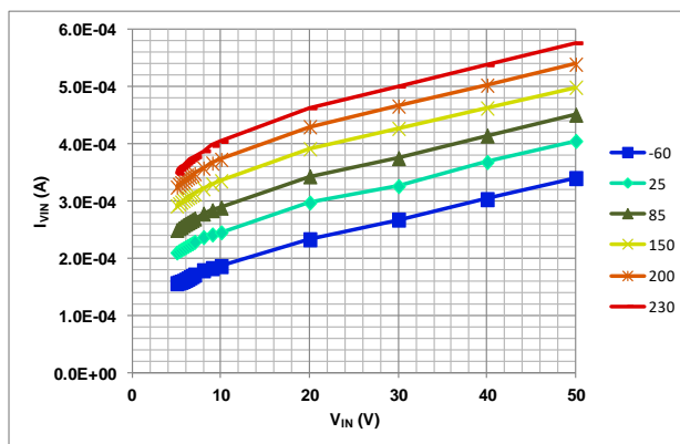
Figure 6. Current through V_{IN} vs input voltage ( V_{IN} ) for different case temperatures with V_{DD}=5V supplied by external source through pin VOUT. Synchronous mode (PSkipEnbl=AsyncEnbl=0), /LPMODE=0, Freq=520kHz, load capacitance on HDrv and LDrv 200pF.
