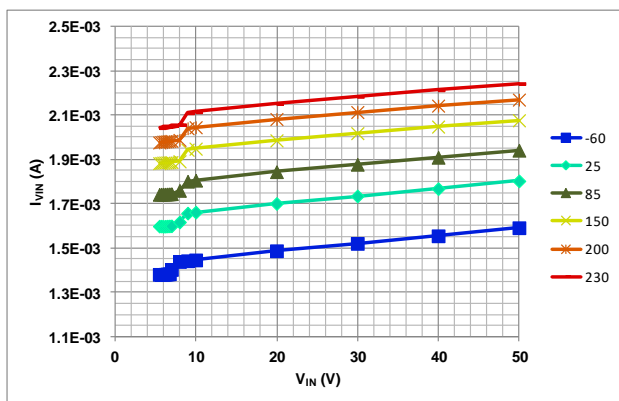
Figure 5. Current through V_{IN} vs input voltage ( V_{IN} ) for different case temperatures. Synchronous mode (PSkipEnbl=AsyncEnbl=0), V_{DD}=4V (/LPMODE=0), Freq=510kHz, load capacitance on HDrv and LDrv 200pF.
