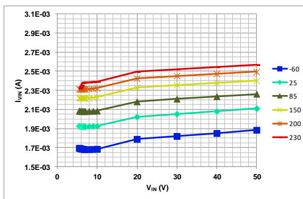
Figure 4. Current through V_{IN} vs input voltage ( V_{IN} ) for different case temperatures. Asynchronous mode (AsyncEnbl=1) without pulse slipping (PSkipEnbl=0), V_{DD}=5V (/LPMODE=1), Freq=520kHz, load capacitance on HDrv and LDrv 200pF.
