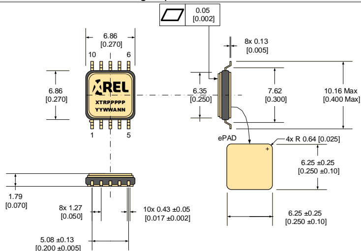
Gull-wing flat pack with ePad CDFP10
