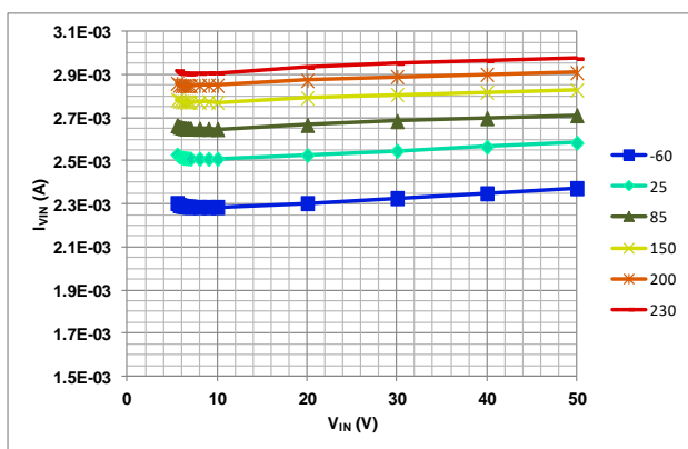
Figure 3. Current through V_{IN} vs input voltage ( V_{IN} ) for different case temperatures. Synchronous mode (PSkipEnbl=AsyncEnbl=0), V_{DD}=5V (/LPMODE=1), Freq=520kHz, load capacitance on HDrv and LDrv 200pF.
