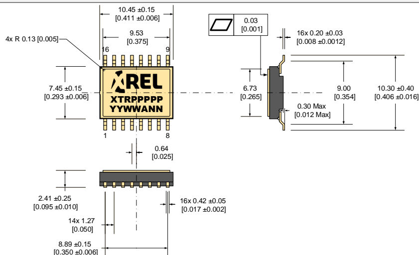
Ceramic Small Outline IC SOIC16
