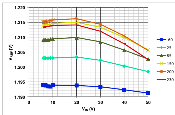
Figure 2. Reference voltage vs input voltage ( V_{IN} ) for different temperatures.
