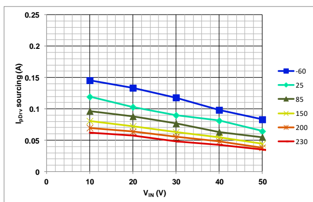
Figure 21. Peak sourcing current capability of output drivers vs input voltage ( V_{IN} ) for different case temperatures. V_{DD}=4V (/LPMMode=0).
