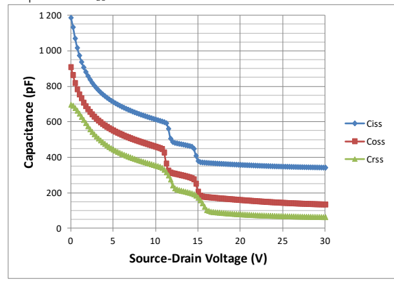
Figure 24. Capacitance vs Source-Drain Voltage at T_c=25^\circ C .
